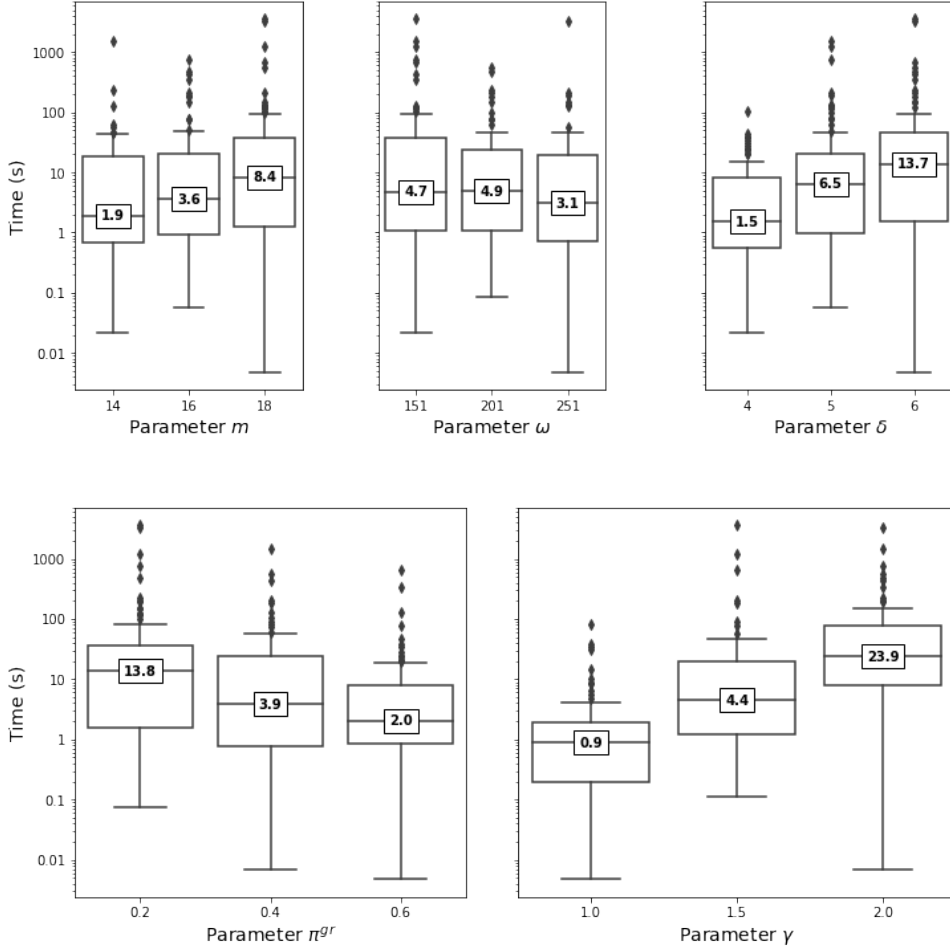
Figure 6: Impact of instance generation parameters on the solution time of model M1 + TASKINC + MINIT .
