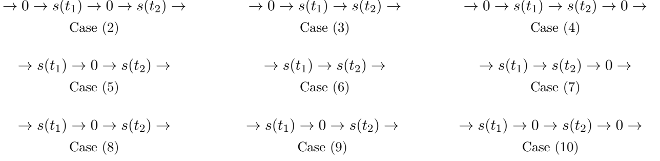
Figure 3: Possible cases for the costs associated with variables y_{t_1, j_1, t_2, j_2} . Each case depicts more movements than those considered in the corresponding cost; this is because doing otherwise would lead to count some movement costs twice.
