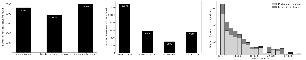
Figure 9: Number of times each destroy (left) and repair (centre) method was used to produce a new best solution during the long (30 minutes) runs. The rightmost chart reports the iteration numbers, grouped in twenty bins, at which new best solutions have been found. Each bar is decomposed by instance size (medium or large) and the y axis is logarithmic. In all charts, the first one thousand iterations of each run have been disregarded.
