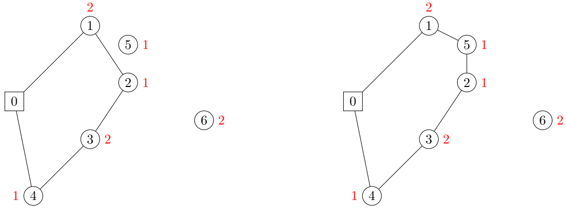
(a) An initial tour and two possible customers to insert. Red numbers indicate prizes.
