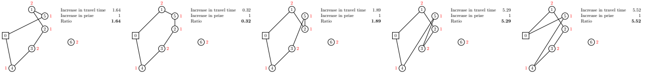
(c) Possible insertions of customer 5 and relative calculations of the ratio between increased travel time and increased profit.
