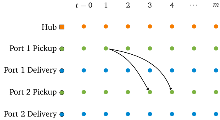
(c) The time-expanded graph for a particular vessel, where each node is copied once for each time instant. Two arcs are depicted, representing sailing between two ports at different speeds.
